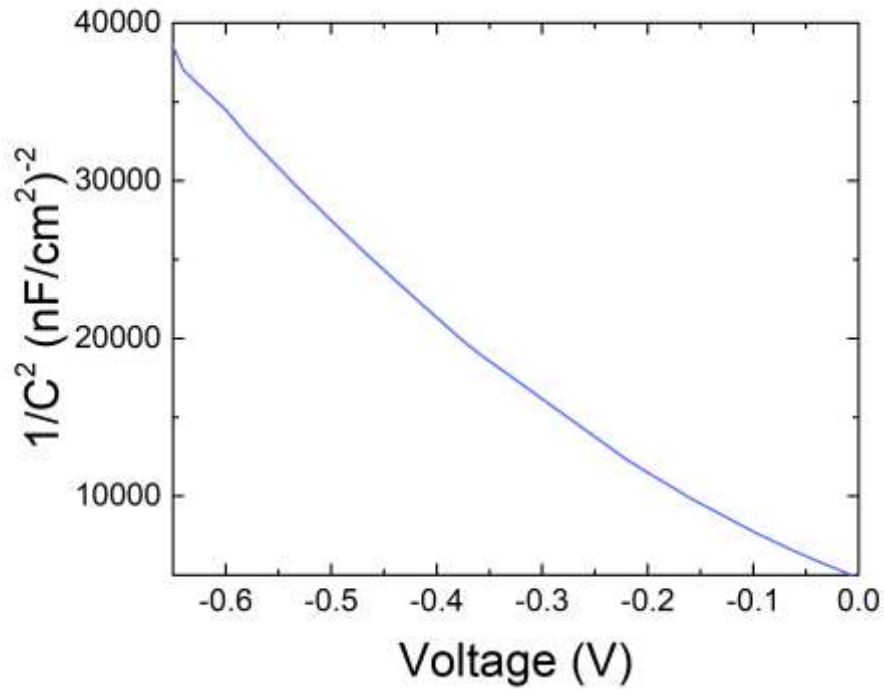
Fig. 4. Mott-Schottky plot.
