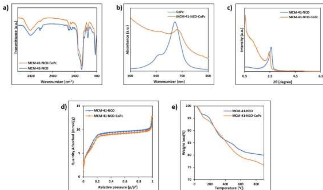
Figure 1. Characterization data of MCM-41-NCO and MCM-41-NCO-CoPc, a) FT-IR spectra, b) UV-Vis. and solid-state UV-Vis. spectra, c) XRD powder patterns, d) N 2 sorption isotherm, e) TGA thermographs
