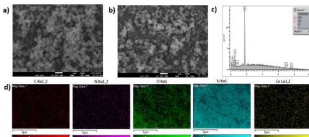
Figure 2. a) SEM micrograph of MCM-41-NCO, b) SEM micrograph of MCM-41-NCO-CoPc, c) EDS analysis of MCM-41-NCO-CoPc, d) EDS mapping of MCM-41-NCO-CoPc
