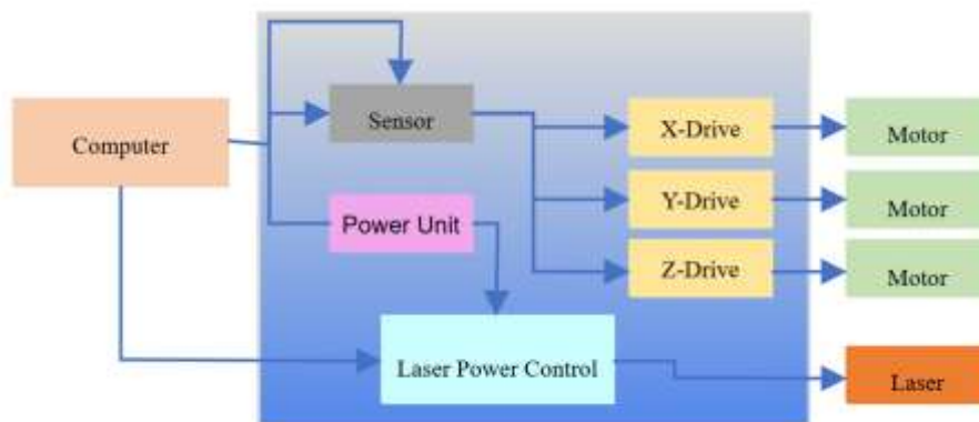
Figure 2: The system's block diagram.
