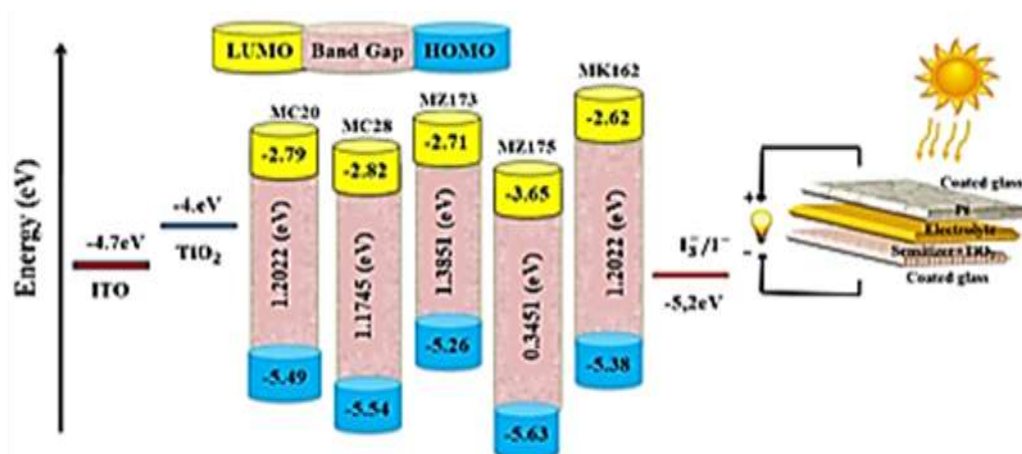
Fig. 1. Energy level of the studied compounds.
