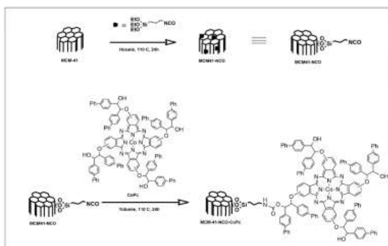
Scheme 1. Synthesis steps of the heterogeneous catalyst MCM-41-NCO-CoPc
